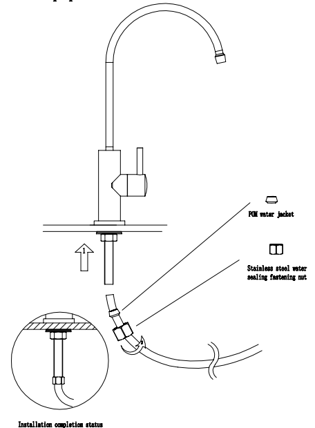
Step 4: direct drinking water pipe installation
